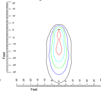
Mounting at 25'
