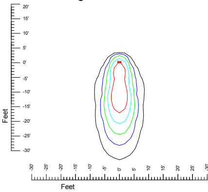
Mounting at 20'
