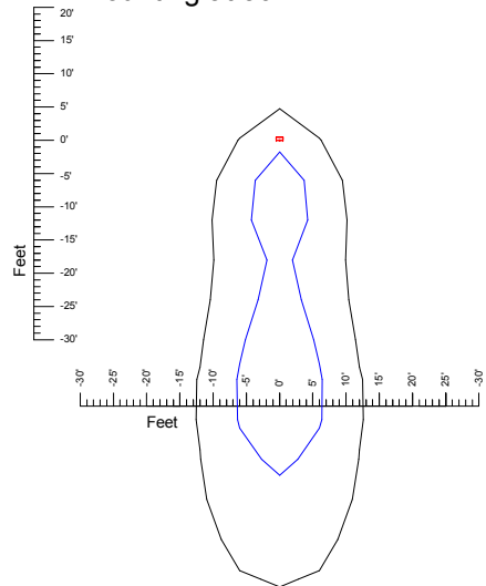
Mounting at 30'
