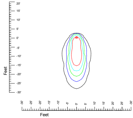
Mounting at 15'
