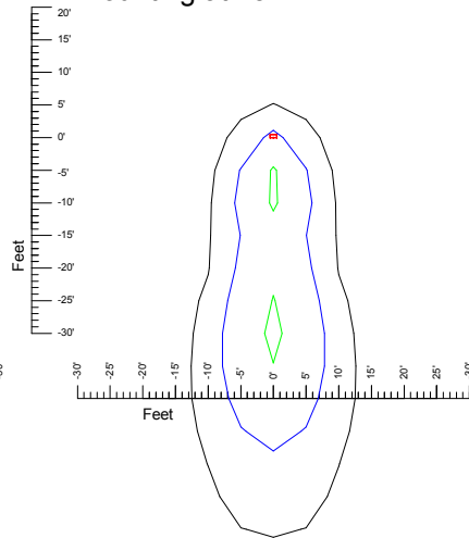
Mounting at 25'
