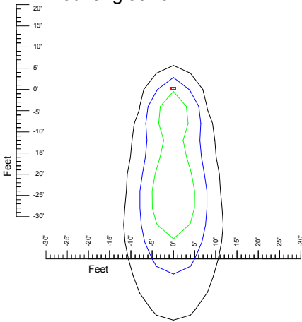
Mounting at 20'
