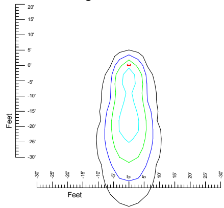
Mounting at 30'
